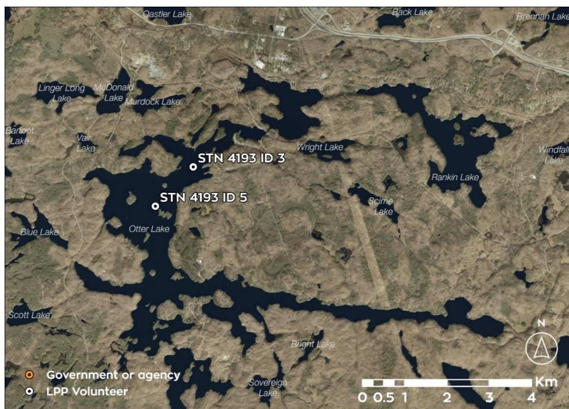
Figure 5. Active and recently active Otter Lake LPP sampling locations. Site ID 5 location is approximate.
